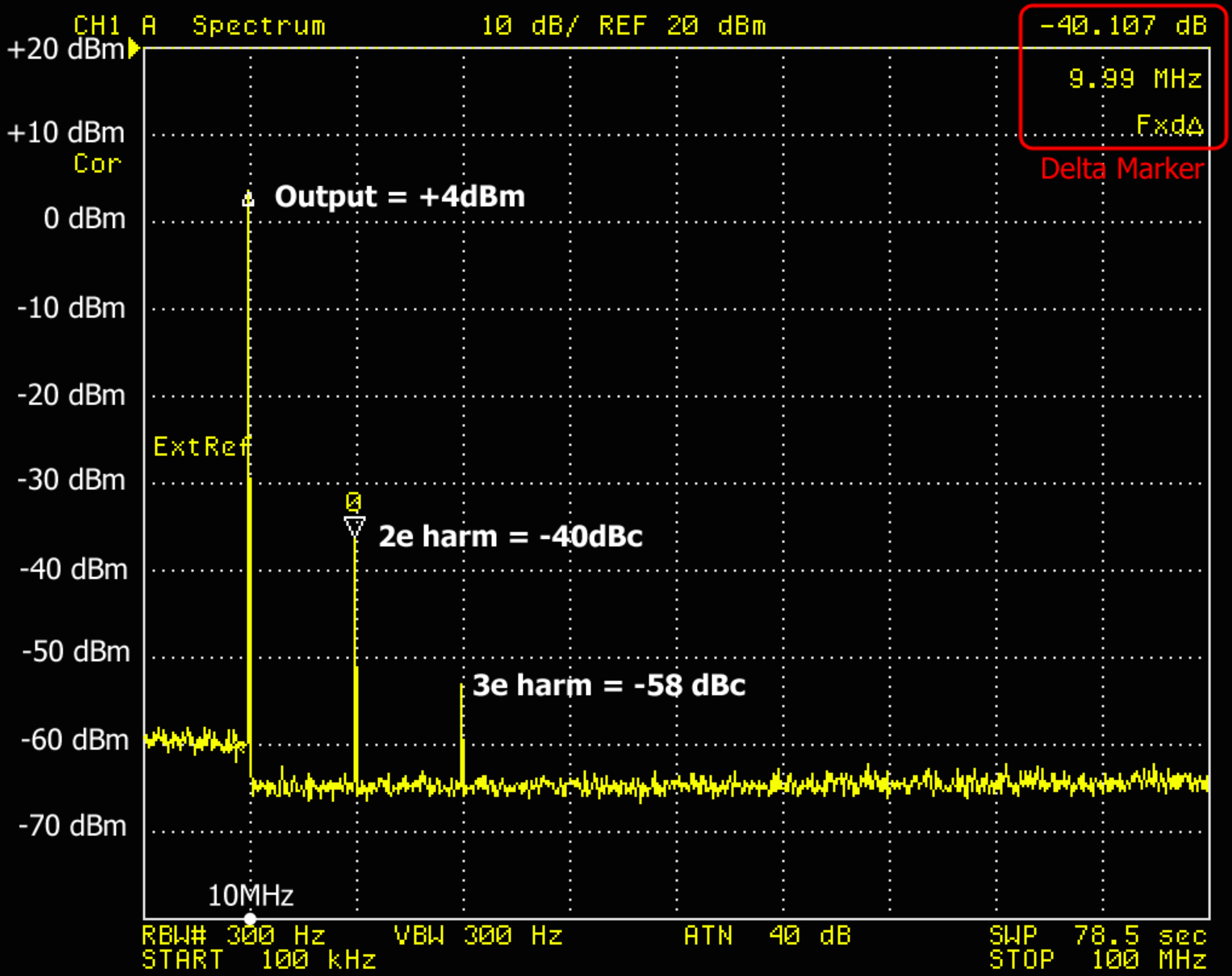
OCXO Oscilloquartz 8663-XS nr.1 (sn.17702) output & harmonischen
