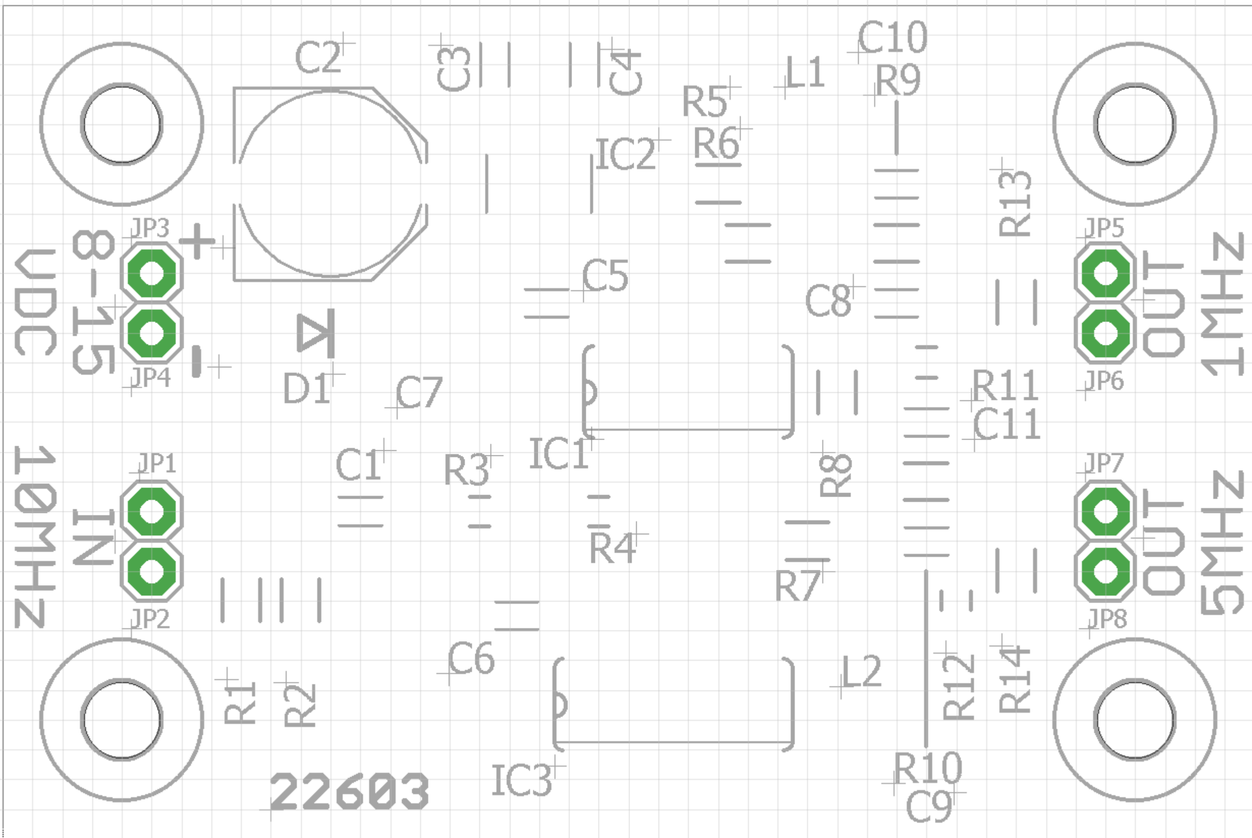
10MHz Reference divider v1.0
