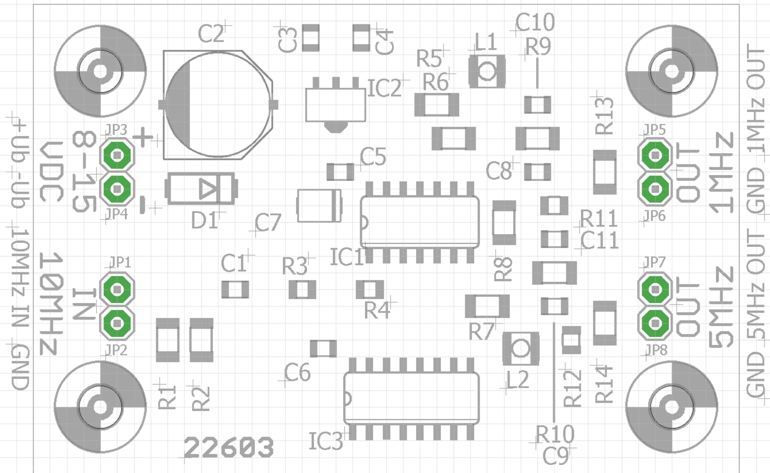
10MHz Reference divider v1.0 Top Component names
