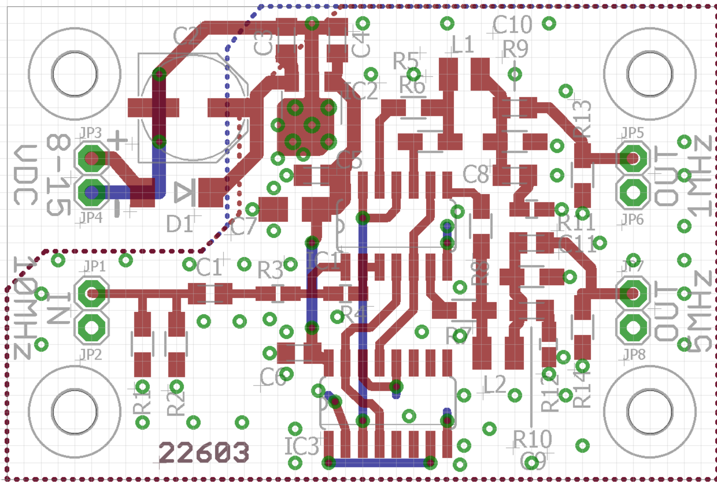
10MHz Reference divider v1.0 Top + Bottom copper
