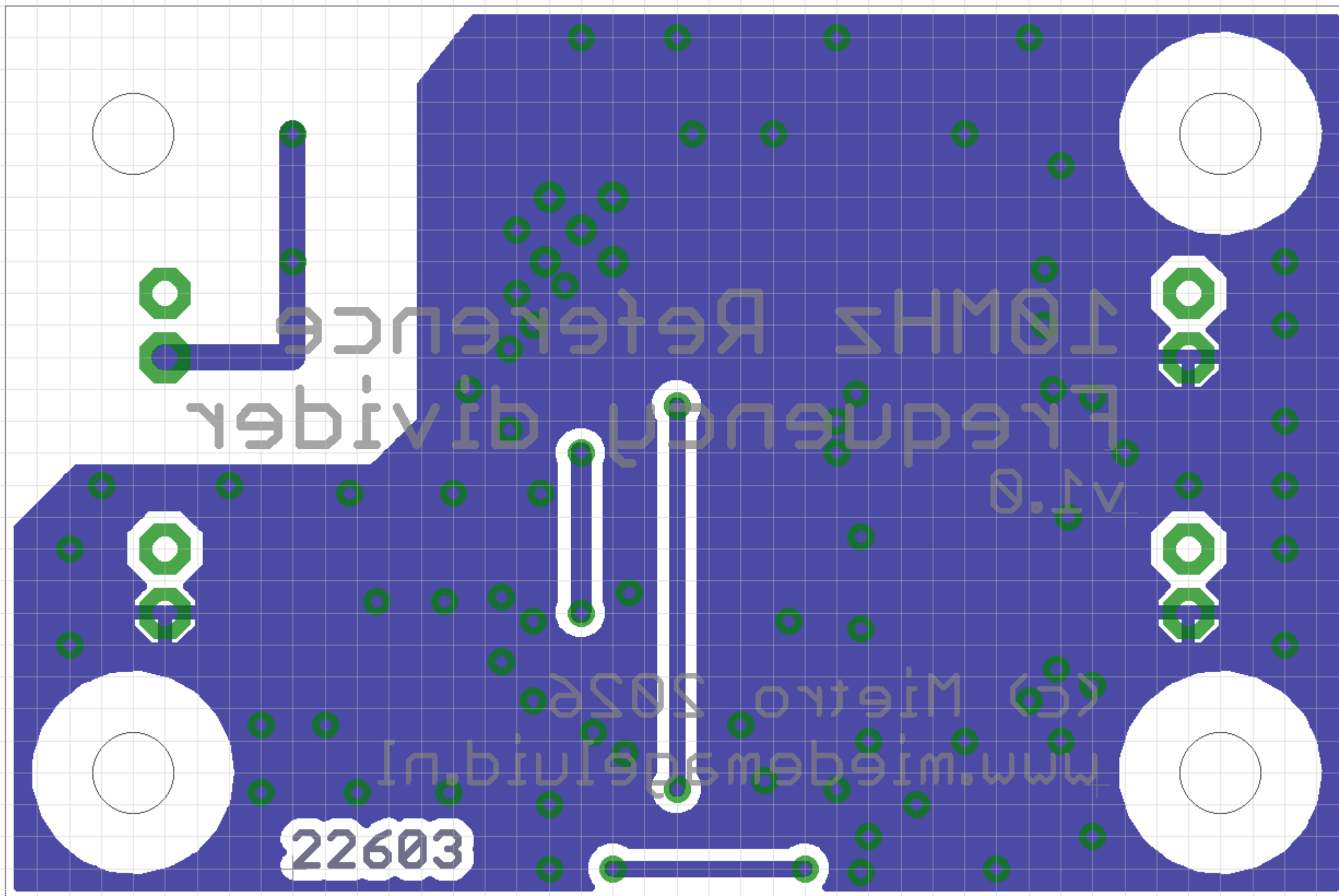
10MHz Reference divider v1.0 Bottom copper with fill
