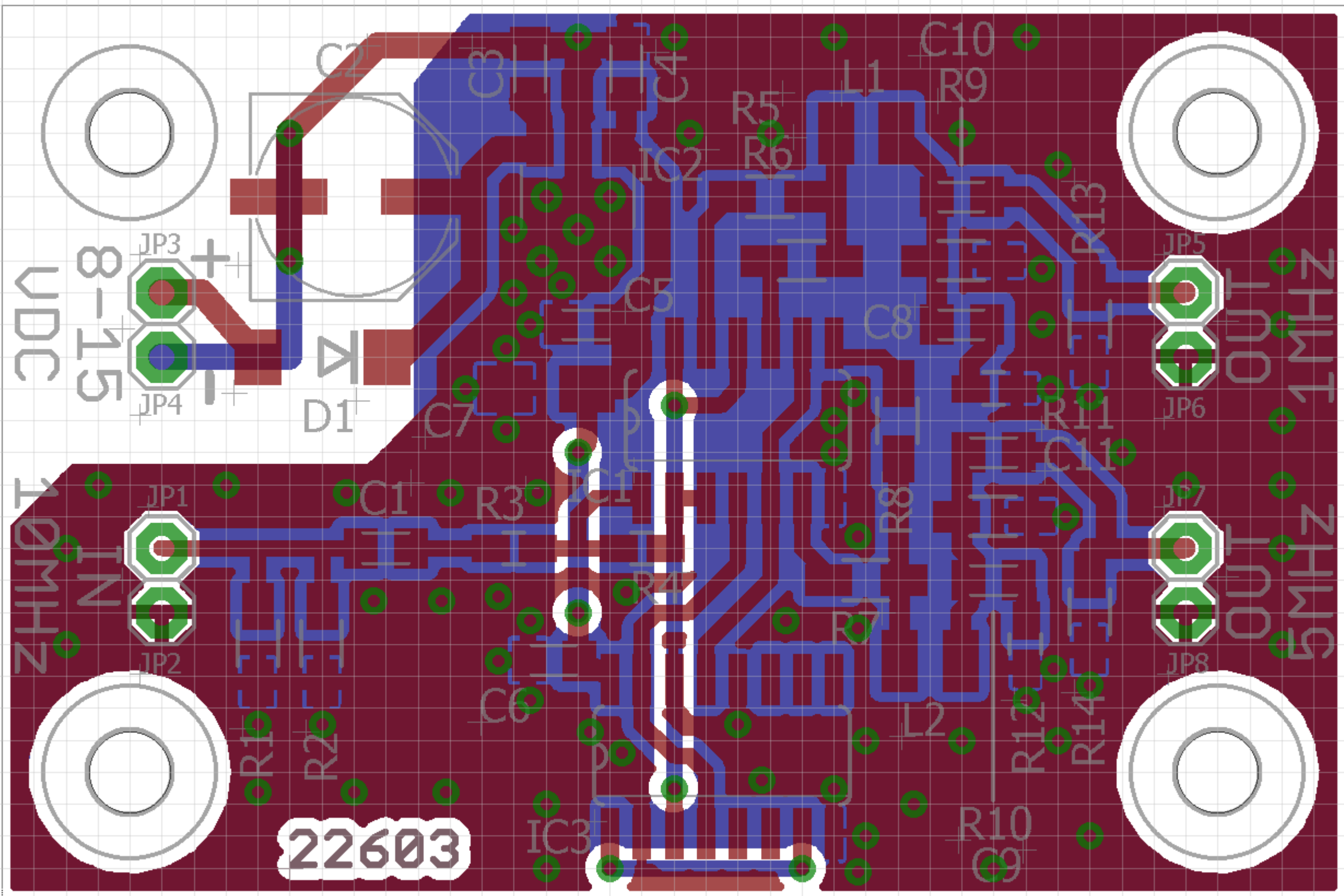
10MHz Reference divider v1.0 Top + Bottom copper with fill
