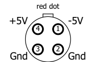
4-pin Lemo power connector
