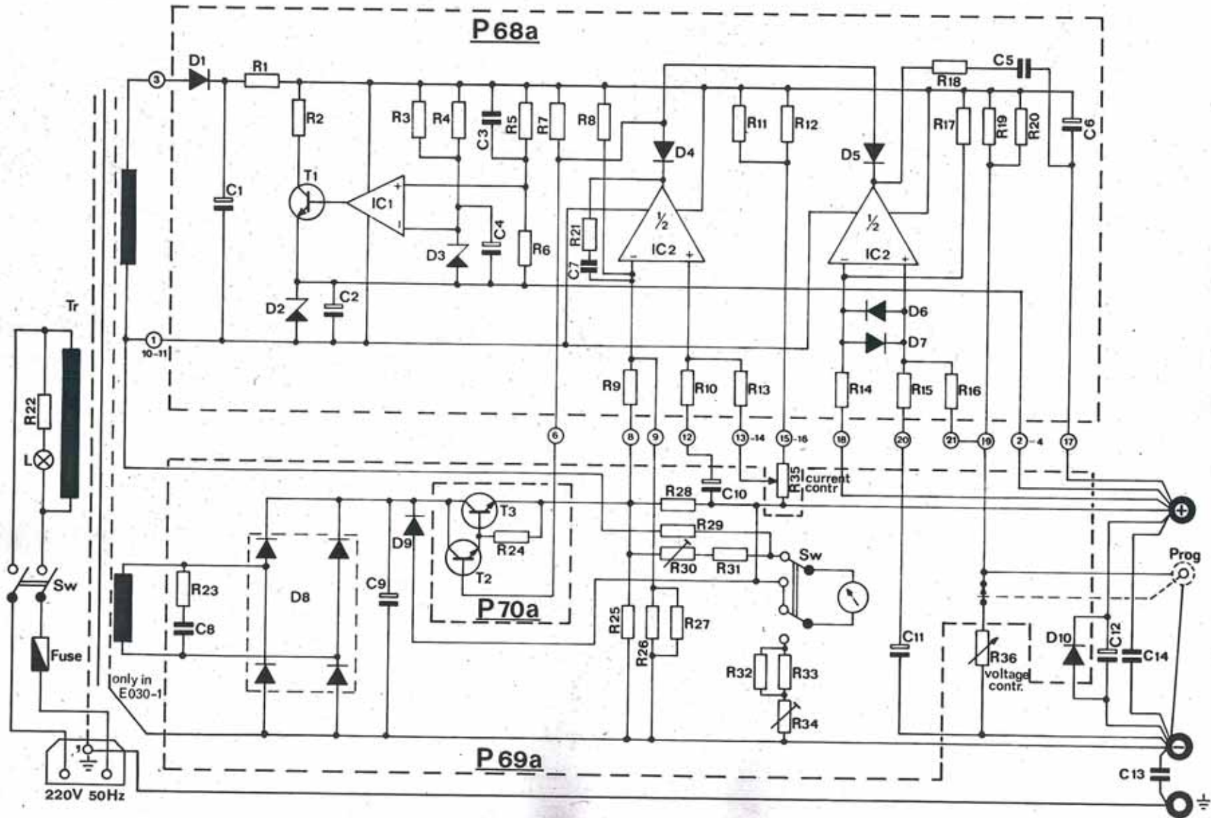
circuit diagram E 015 - 2 , E 030 - 1 , E 060 - 0.6 serial no 6939 and up
