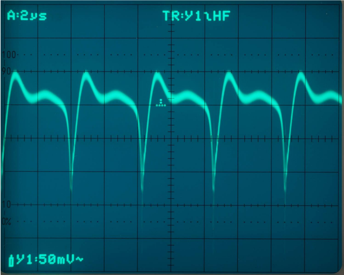
muRata DC-DC - U_{in} , zonder filters (load 2x50mA)
