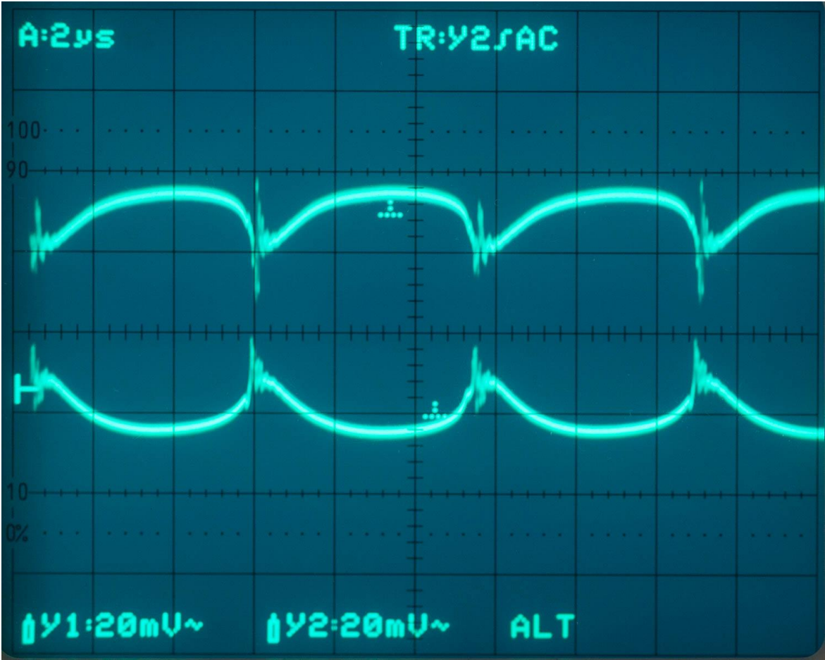
XP power DC-DC - Uuit zonder filters (load 2x50mA)
