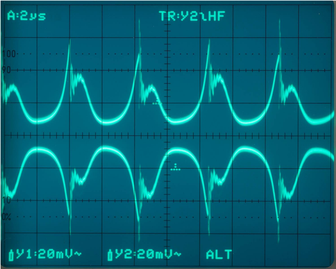
muRata DC-DC - Uuit zonder filters (load 2x50mA)
