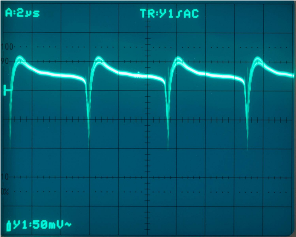
XP Power DC-DC - U_{in} zonder filters (load 2x50mA)
