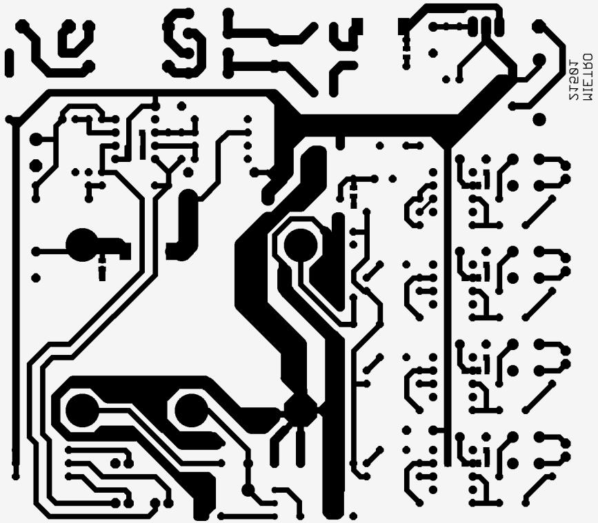
E730858 BOTTOM layer Image (topview)
